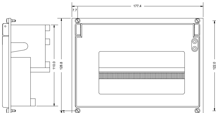
Overall printer dimensions
